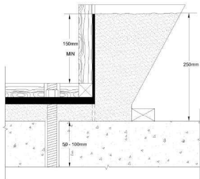
Fig.2 : Typical hopper system
